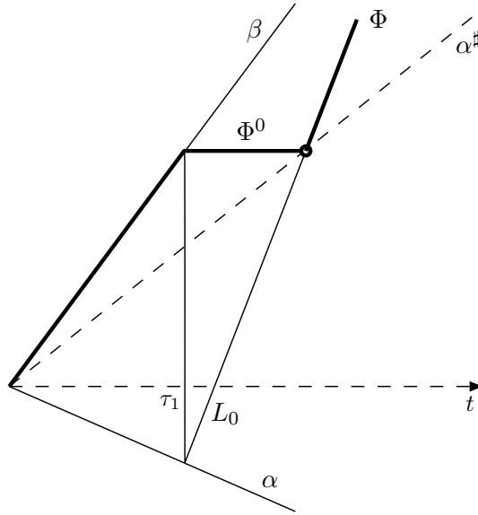
FIGURE 5. Sketch of the proof of Lemma 6.2 ( \sigma = 0 )
