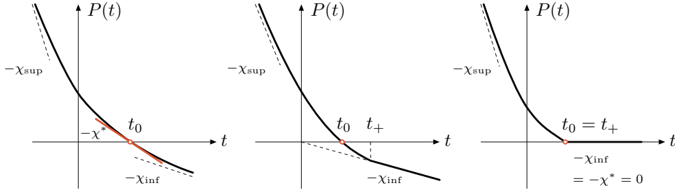
FIGURE 1. The geometric pressure: LyapHyp with t_+ = \infty , LyapHyp with t_+ < \infty , and non-LyapHyp
