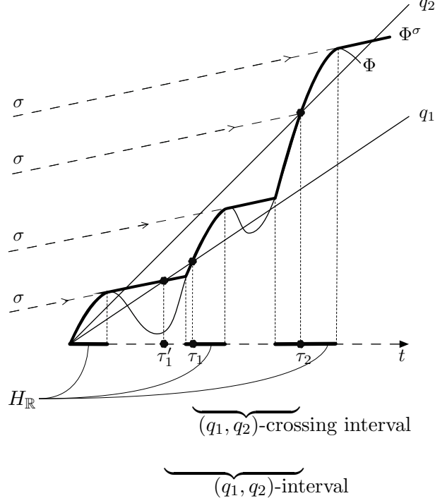
FIGURE 4. (q_1, q_2) - and crossing intervals
