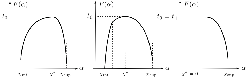
FIGURE 2. F(\alpha) : LyapHyp with t_+ = \infty , LyapHyp with t_+ < \infty , and non-LyapHyp
