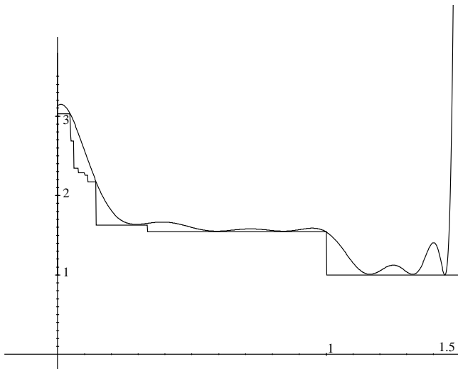
Fig. 1. Comparison of \theta_{210}^* and the optimizing polynomial
