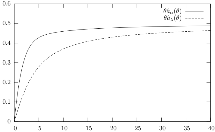
Fig. 2. The functions \theta \mapsto \theta\hat{a}_\lambda(\theta) and \theta \mapsto \theta\hat{a}_\alpha(\theta)
