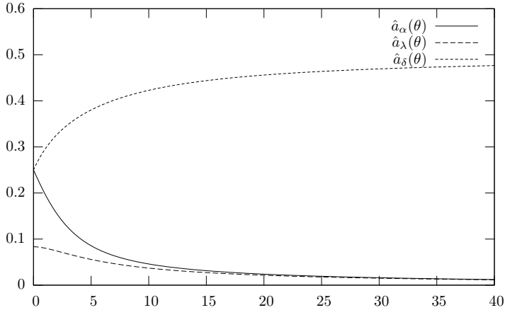
Fig. 1. The functions \hat{a}_\lambda , \hat{a}_\delta and \hat{a}_\alpha as functions of \theta
