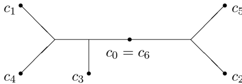
Fig. 1. The abstract Hubbard tree for \nu = \overline{10110^*} . The three branch points form a period 3 orbit, but the third iterate permutes the arms in a non-cyclic way. As a result, this tree is not the Hubbard tree of any quadratic Julia set.
