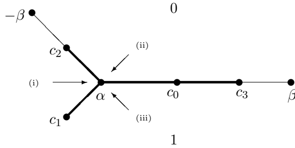
Fig. 2. A Hubbard tree for \nu = 110\bar{1} (in bold lines) and its extension. The third image of the critical value is the fixed point \alpha , which in this case has three external approaches, so c_1 has three external angles.
