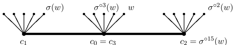
Fig. 3. The extended Hubbard tree for \nu = \overline{10^*} and \widehat{V} = \{\sigma^{oi}(w) : i \geq 0\} with w = (110)^n 0^* \nu for n = 5 . The Hubbard tree is in bold lines.
