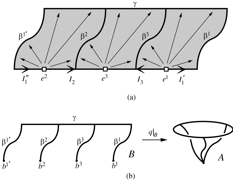
Fig. 4. A deformation retraction of K \setminus \{\bar{e}\}
