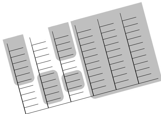
Fig. 1. A block of the barrier [\omega]^2
