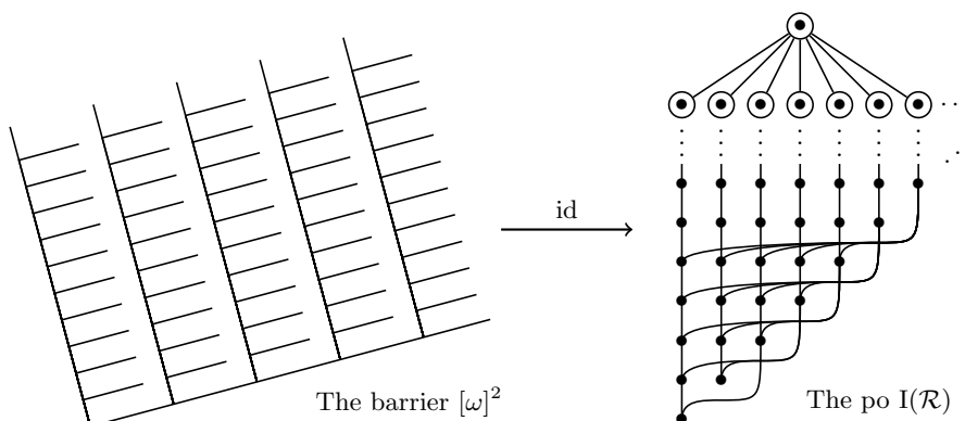
Fig. 2. A bad Cauchy supersequence in Rado's poset
