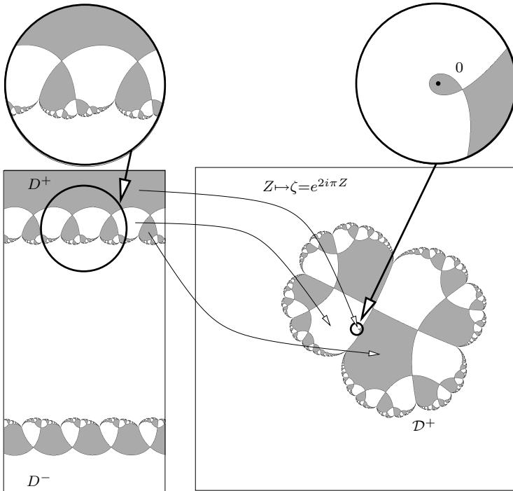
Fig. 4. Left: The tiled domains D^+ and D^- . Right: the tiled domain D^+ .
