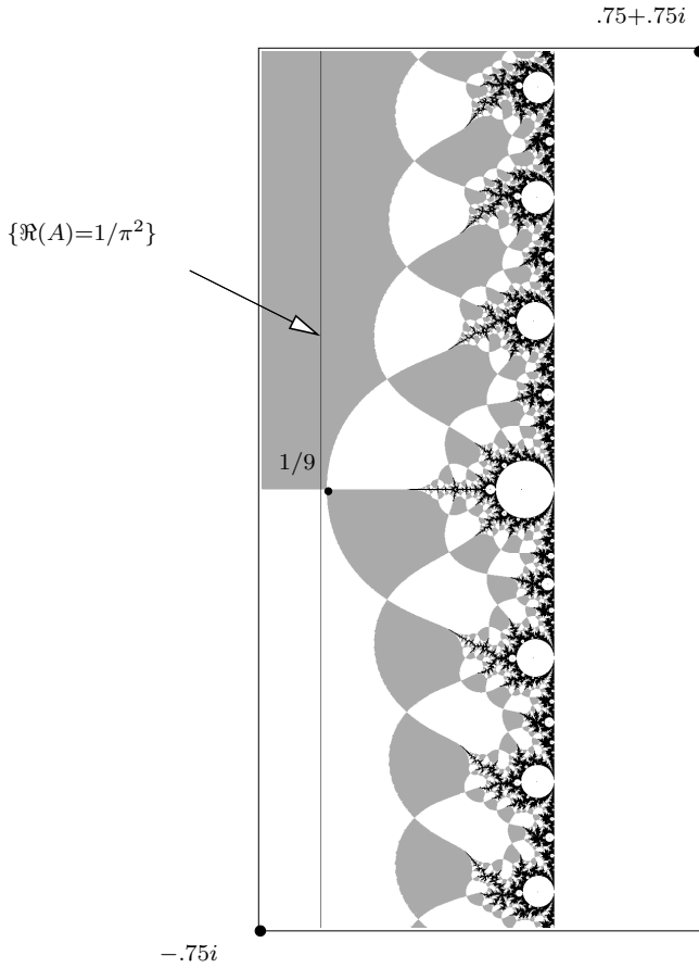
Fig. 11. Critical orbit relations for quadratic rational maps with a multiple fixed point: Z \mapsto Z + 1 + A/Z .
