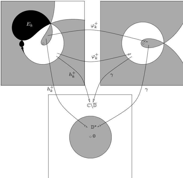
Fig. 10. The relation h_k^\pm = \gamma \circ \varphi_k^\pm
