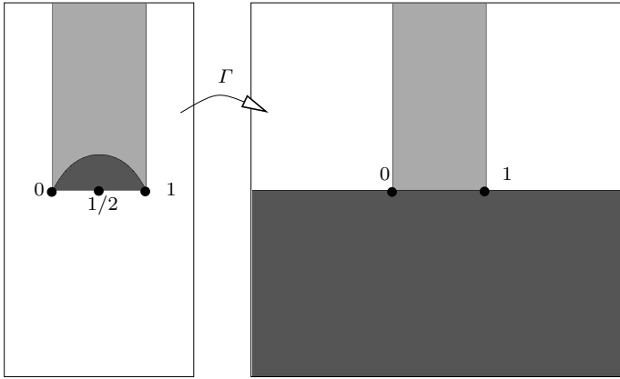
Fig. 9. The isomorphism \Gamma : \{Z \in \mathbb{H}^+ \mid 0 < \Re(Z) < 1\} \rightarrow \mathbb{H}^- \cup \{Z \in \mathbb{C} \mid 0 < \Re(Z) < 1\}
