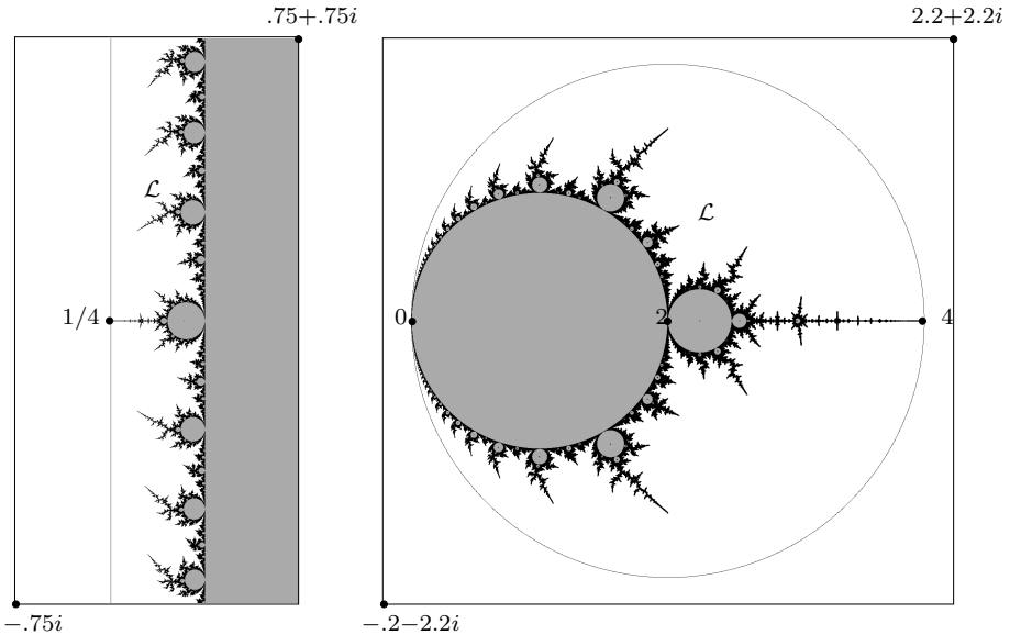
Fig. 6. The connectedness locus \mathcal{L} of the family \{Z \mapsto Z + 1 + A/Z\} , A \in \mathbb{C}^* . Left: in the coordinates A . Right: in the coordinates 1/A .
