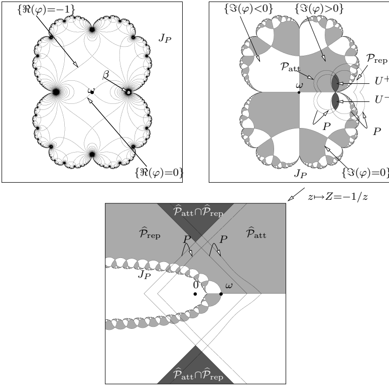
Fig. 3. The polynomial P(z) = z + z^2 has a parabolic fixed point at 0 with immediate basin \Omega . Any attracting Fatou coordinate extends to a ramified covering \varphi_{\text{att}} : \Omega \rightarrow \mathbb{C} . We can normalize \varphi_{\text{att}} so that \varphi_{\text{att}}(\omega) = 0 , where \omega = -1/2 is the unique critical point of P . Left: the curves \{z \in \Omega \mid \Re(\varphi_{\text{att}}(z)) \in \mathbb{Z}\} . Right: the basin \Omega is tiled by the regions \{z \in \Omega \mid \Im(\varphi_{\text{att}}(z)) < 0\} and \{z \in \Omega \mid \Im(\varphi_{\text{att}}(z)) > 0\} . Down: the same picture in the coordinate Z = -1/z .
