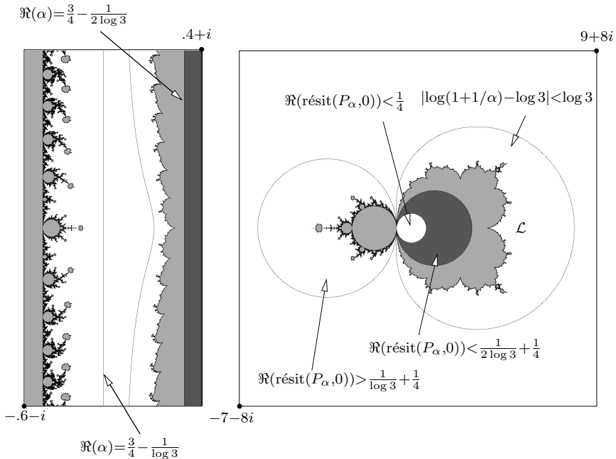
Fig. 7. The connectedness locus of the family P_\alpha(z) = z + z^2 + \alpha z^3 . Left: in the coordinate \alpha . Right: in the coordinate 1/\alpha .
