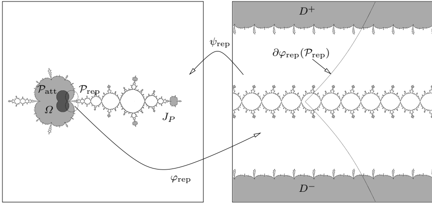
Fig. 2. The polynomial P(z) = z + z^2 - .46z^3 has a parabolic fixed point at 0. Left: the Julia set of the polynomial P . The parabolic basin of 0 is colored grey. Right: the preimage of J_P by the meromorphic function \psi_{\text{rep}} : \mathbb{C} \rightarrow \mathbb{P}^1 .
