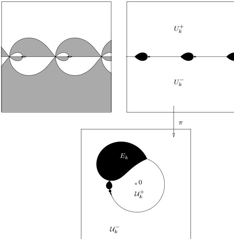
Fig. 8. The sets U_k^\pm , \mathcal{U}_k^\pm and E_k
