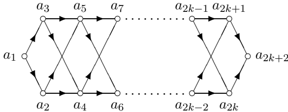
Fig. 3. A k -elongated partition diamond of length 1
