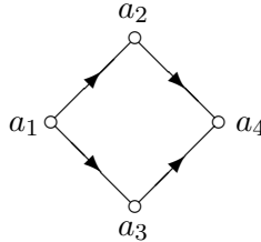
Fig. 1. The inequalities (1.1)
