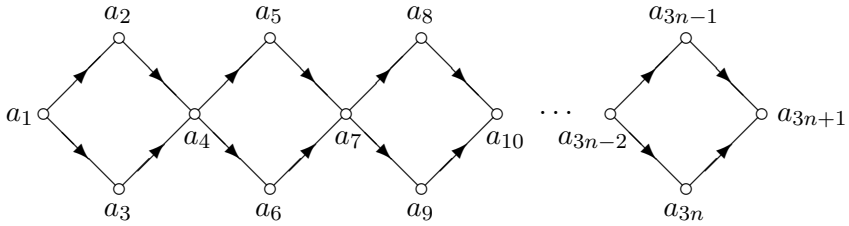
Fig. 2. A plane partition diamond of length n
