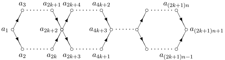
Fig. 4. A k -elongated partition diamond of length n
