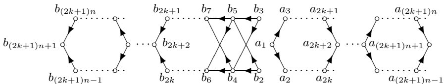
Fig. 5. A broken k -diamond of length 2n
