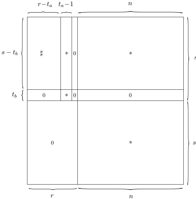
Figure 2. The shape of a 2s \times (n + r) matrix
