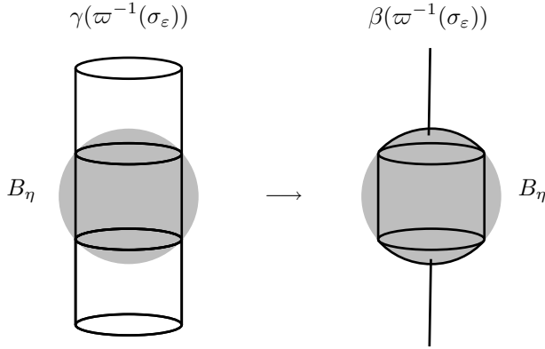
Figure 1. Homotopy from \gamma|\varpi^{-1}(\sigma_\varepsilon) to \beta
