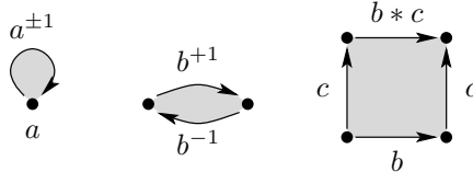
Fig. 2. Elementary homotopies for paths in P(Q)
