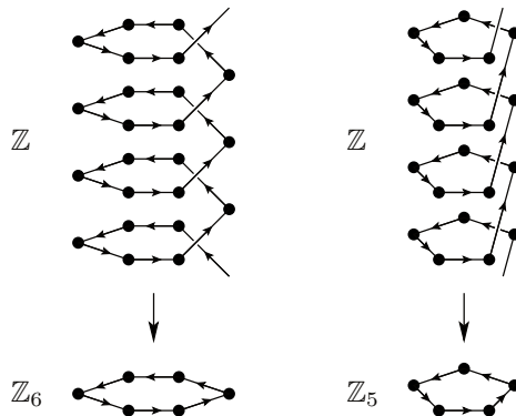
Fig. 1. The universal covering of the quandle Q_{6,5}
