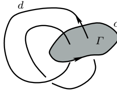
Fig. 1. Here \text{lk}(c, d) = +2 .
