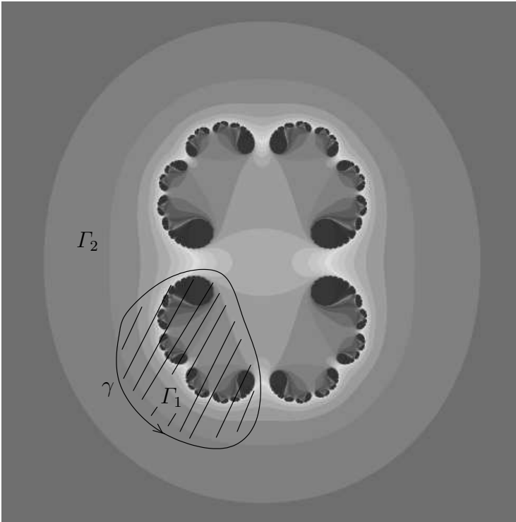
Fig. 2. Both choices \Gamma_1 (inside of \gamma ) and \Gamma_2 (outside of \gamma ) yield the same \text{lk}(\gamma, T) .
