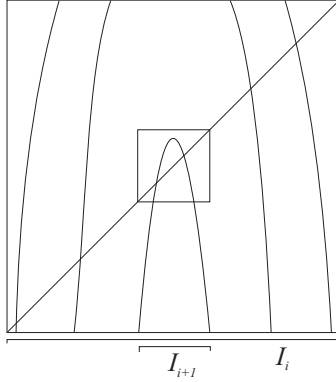
Fig. 1. F_i is high and central
