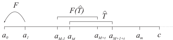
Fig. 2. When \widehat{T} intersects the boundary points \partial I_j
