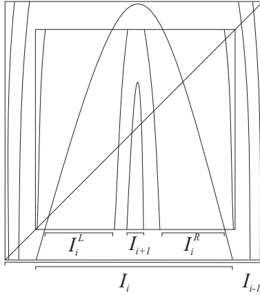
Fig. 3. The exceptional case
