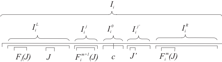
Fig. 4. An illustration of Proposition 5.3
