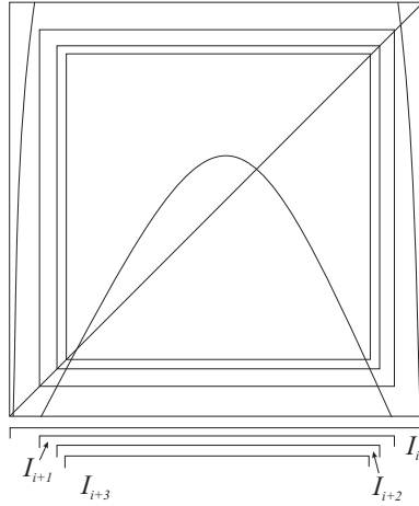
Fig. 5. An infinite cascade
