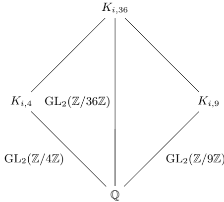
Fig. 2. Decomposition of the 36-division fields for E_i
