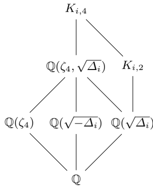
Fig. 3. A portion of the subfield diagram of K_{i,4} from [1, Figure 5.7]
