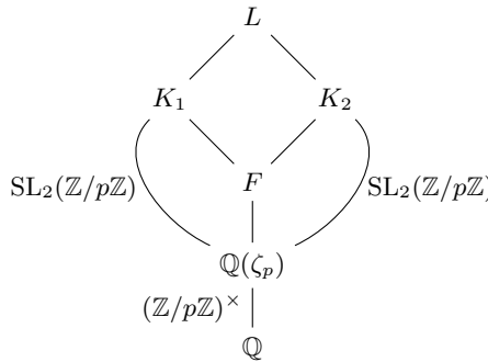
Fig. 1. Division fields for p \geq 5
