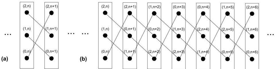
Fig. 1. (a): A drawing of a segment of the Cayley graph for \Gamma_3 . Rectangles represent sets on which the induced subgraph is complete, so the edges within them are not drawn. (b): Same as (a), but for \Delta_3 , and realized using the isomorphism \phi_k .
