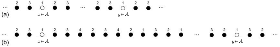
Fig. 3. A drawing of the coloring procedure for \Delta'_3 . Points are arranged in a line on the page according to some natural \mathbb{Z} -order for their connected component. Hollow points represent a single point, while filled-in ones represent two adjacent (in the \mathbb{Z} -order) ones having the same color. The numbers over the points denote the colors. x and y are as in the proof of the theorem. (a): The case where \prec_x = \prec_y . (b): The case where \prec_x \neq \prec_y .
