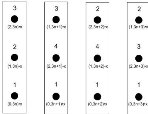
Fig. 2. An example of the technique for going from \sigma_n to \sigma_{n+1} = \rho_{n+1}\sigma_n . Here k = 3 , \sigma_n = \text{id} , and \rho_{n+1} = (2 \ 3) . The numbers over each point are the colors. The rectangles have the same meaning as in Figure 1. Edges between \mathbb{Z}/k\mathbb{Z} -orbits are omitted. The action of (0, 1) sends each point to its immediate neighbor on the right.
