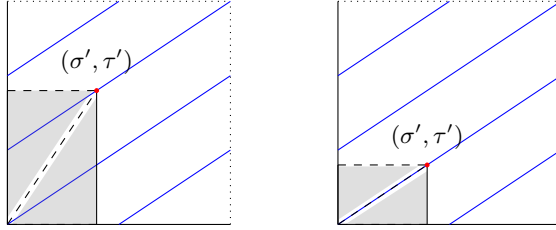
Fig. 7. Solutions to 2x - 3y \in \mathbb{Z} compared to \mathcal{C}'_{\sigma', \tau'} , when k \neq 0 and k = 0
