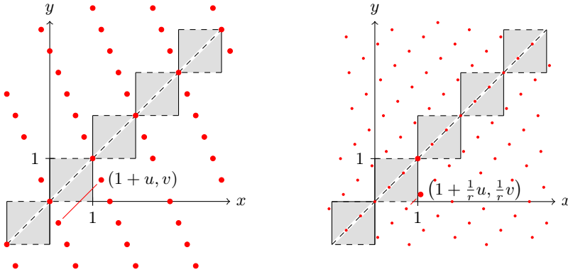
Fig. 4. Lattices \Lambda and \Lambda^{(r)} with r = 3 , shown with punctured approximate diagonal region \mathcal{D}' shaded
