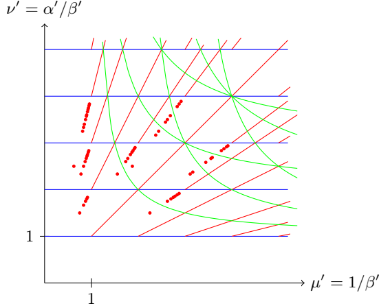
Fig. 2. Negative dilation part of S viewed in (\mu', \nu') -coordinates
