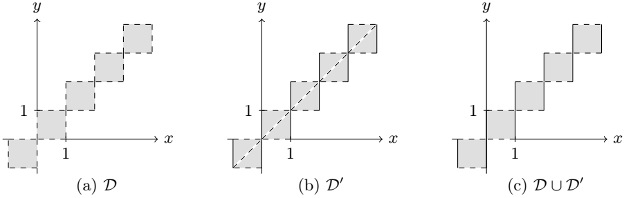
Fig. 3. Regions \mathcal{D} , \mathcal{D}' and \mathcal{D} \cup \mathcal{D}' in \mathbb{R}^2 , in gray
