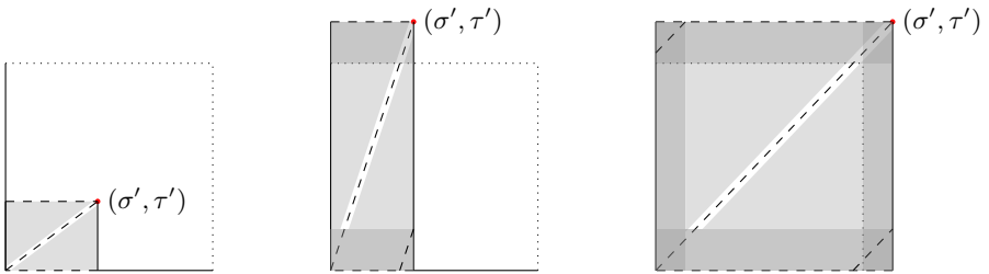
Fig. 6. Modified corner rectangle \tilde{\mathcal{C}}'_{\sigma', \tau'} in the torus \mathbf{T} = \mathbb{R}^2 / \mathbb{Z}^2 , with various (\sigma', \tau')
