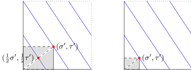
Fig. 8. Solutions to 3x + 2y \in \mathbb{Z} in the torus \mathbf{T} , with k = 2 and k = 1
