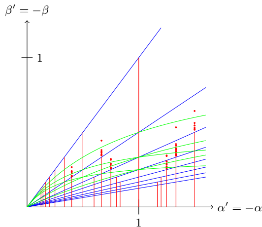
Fig. 1. Negative dilation solutions S' = -S viewed in (\alpha', \beta') -coordinates. Sporadic solutions appear as dots.
