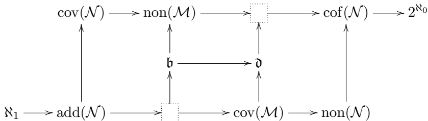
Fig. 1. Cichoń’s diagram with the two “dependent” values removed, which are \text{add}(\mathcal{M}) = \min \{\mathfrak{b}, \text{cov}(\mathcal{M})\} and \text{cof}(\mathcal{M}) = \max \{\text{non}(\mathcal{M}), \mathfrak{d}\} . An arrow \mathfrak{r} \rightarrow \mathfrak{\eta} means that ZFC proves \mathfrak{r} \leq \mathfrak{\eta} .
